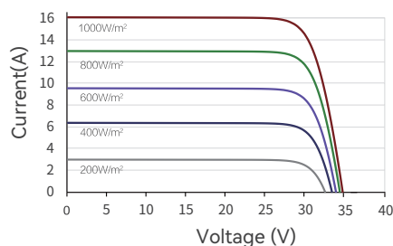
Current-Voltage(455W)
