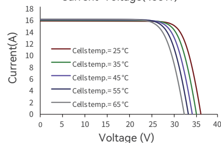
Current-Voltage(455W)
